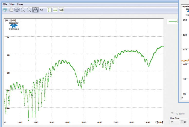
The T3SP1xD series offer S-parameter (S11) measurements up to 15 GHz
